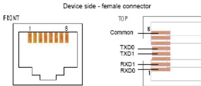
4W- MODBUS on RJ45 connector ( required pin-out )
