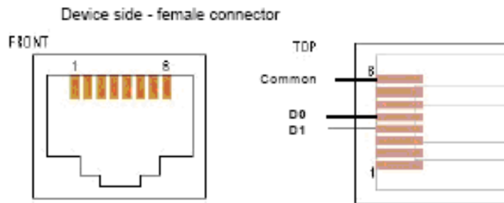
2W- MODBUS on RJ45 connector ( required pin-out )
